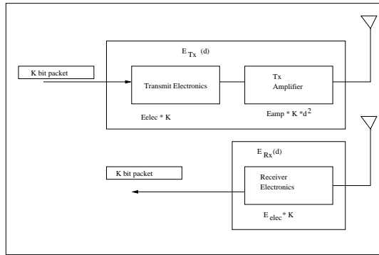
Figure 1. First Order Radio Model
