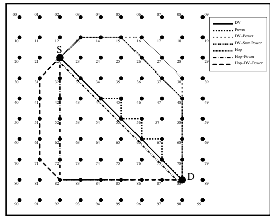
Figure 3. Routing Using Different Metrics at Round 4000
